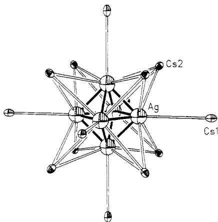
Figure 6. The octahedral \text{Ag}_6 cluster in the large cavity of \text{Ag}_{4.6}\text{Cs}_{13.5}\text{-A} . It is stabilized by coordination to six \text{Cs}^+ ions in a first coordination shell and eight \text{Cs}^+ ions in a second shell. The framework atoms of the large cavity of zeolite A are not shown for clarity. Ellipsoids of 20% probability are shown.
